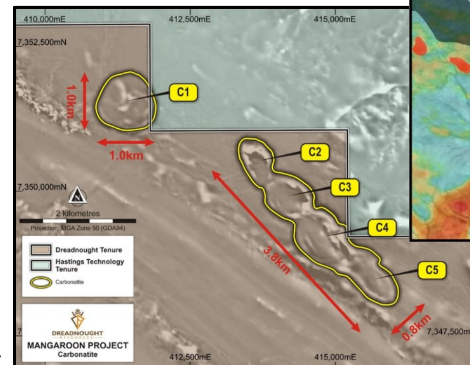
Mangaroon Carbonatite Intrusions (Yin Project) ^
