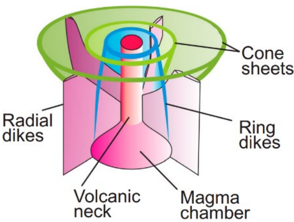
3D carbonatite complex schematic*
