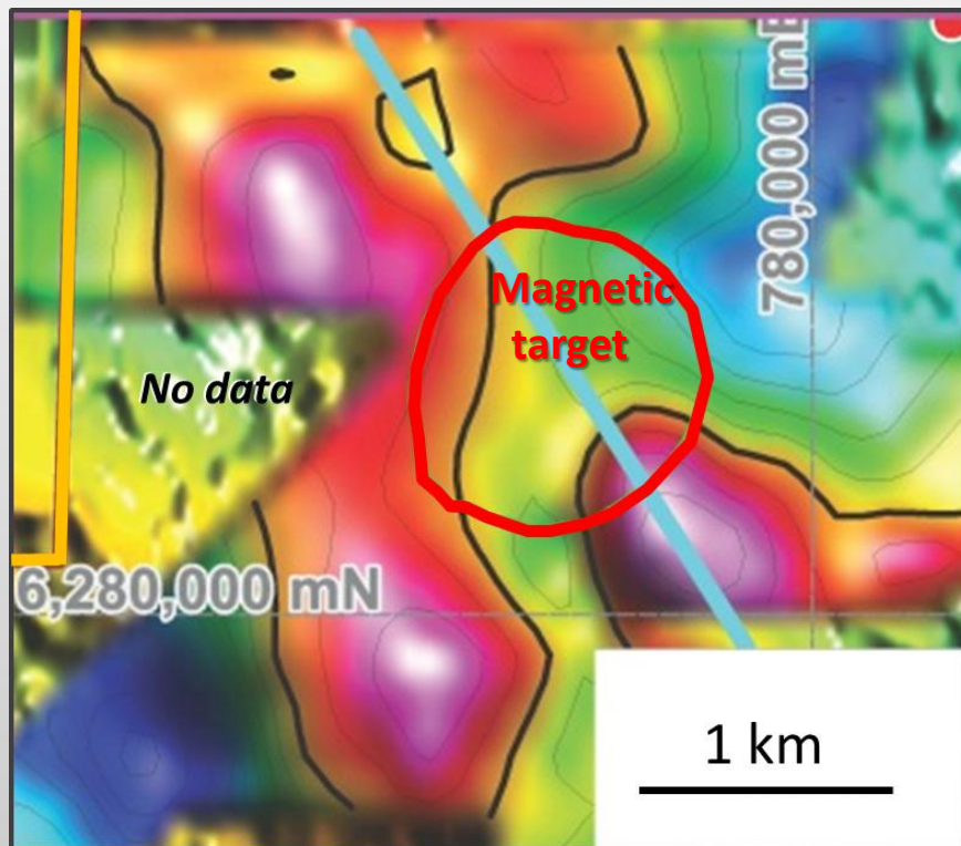
Bouguer gravity image
